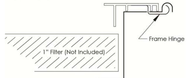
AEC-FG-1 Frame Detail
