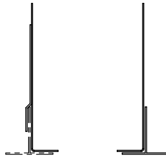
One Pair of TC Clips and One Side T Furnished*
