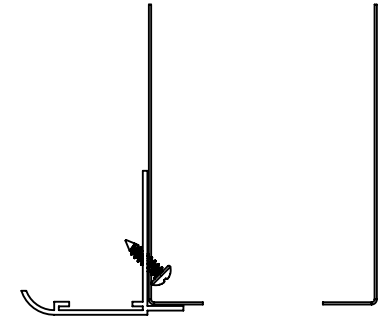
Frame for Concealed Fastening. Shipped Loose. Field Drilled.
