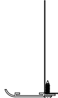
Frame Screwed onto Plenum Lip Using Pan Head Screws. Shipped Loose.
