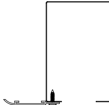
Frame Screwed onto Plenum Lip Using Pan Head Screws. Shipped Loose.
