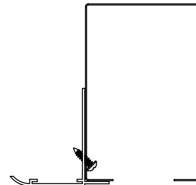
Frame for Concealed Fastening. Shipped Loose. Field Drilled.
